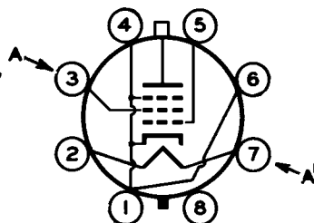
AA'=PLANE OF ELECTRODES
